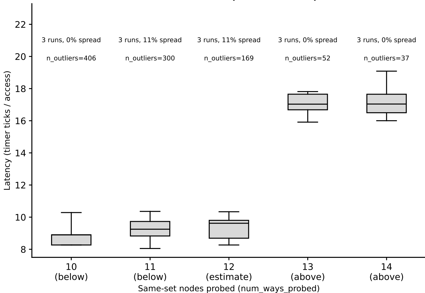
hazel_icelake_6326/phase1_v2: associativity box plots, L3_LLC, random pattern (whiskers = p5/ (Phase I timing-only, auto pipeline) detected associativity estimate: 12-way
