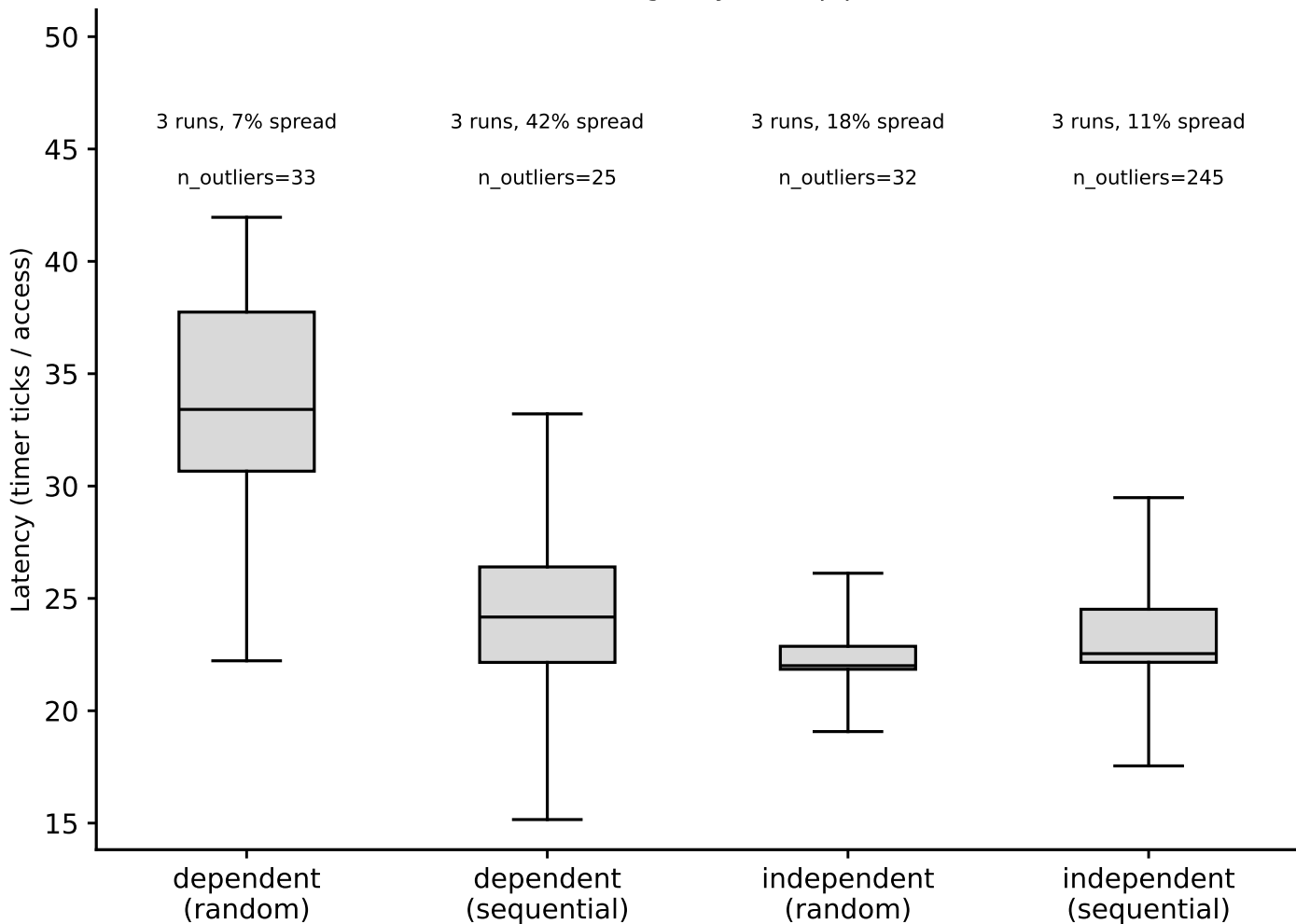
hazel_icelake_6326/phase1_v2: hit-latency box plots, L1 (footprint=64 KiB) (Phase I timing-only, auto pipeline)
