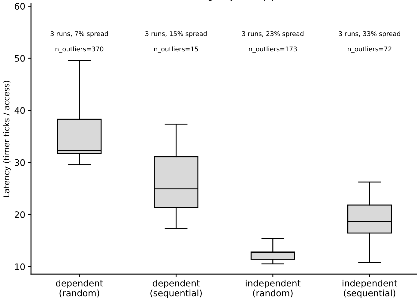
hazel_icelake_6326/phase1_v2: hit-latency box plots, L2 (footprint=1.25 MiB) (Phase I timing-only, auto pipeline)
