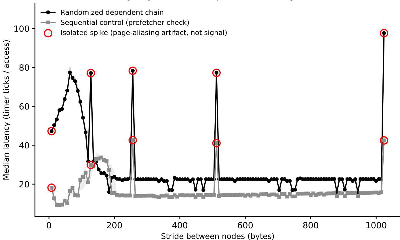
hazel_icelake_6326/phase1_v2: line-size sweep (dependent pointer chase), footprint=2.5 MiB (Phase I timing-only, level boundary=1310720B, single-curve method)
