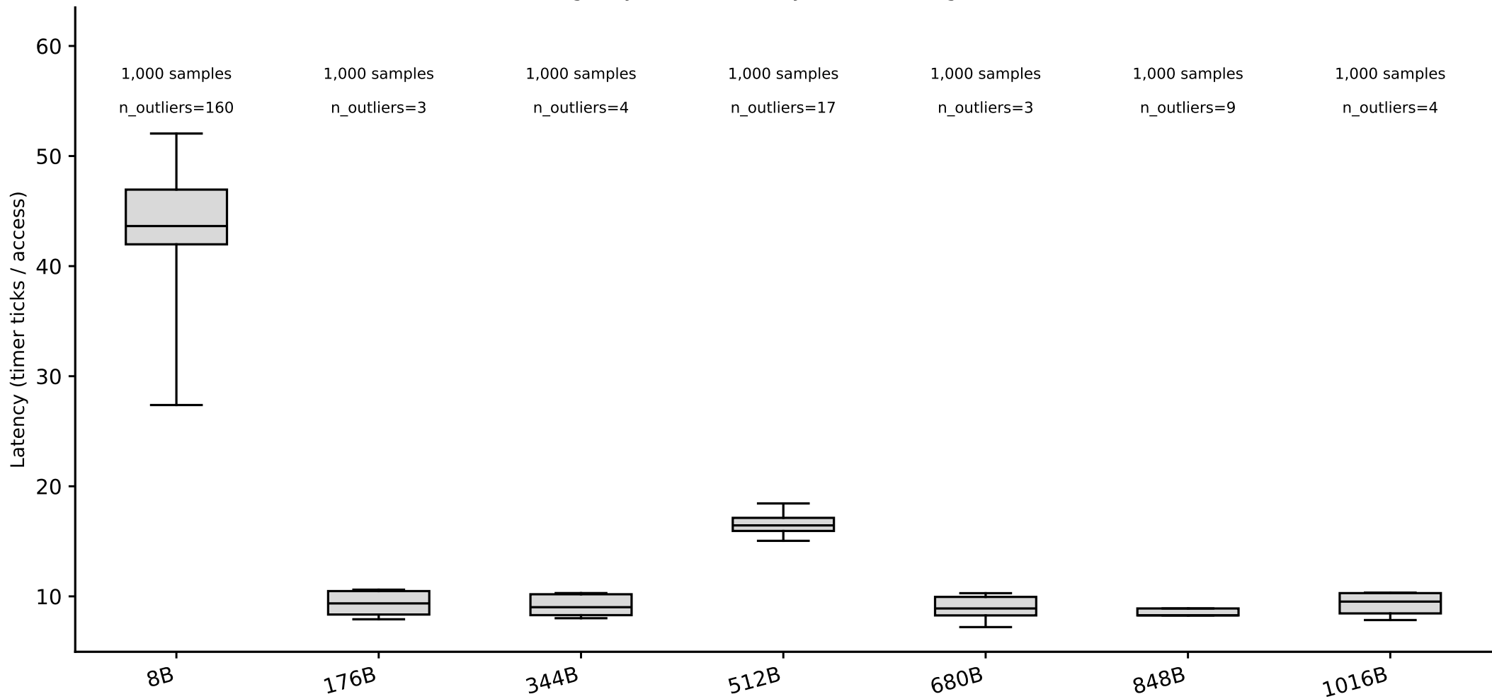
hazel_icelake_6326/phase1_v2: line-size box plots, random pattern (whiskers = p5/p95) (Phase I timing-only, level boundary=65536B, single-curve method)
