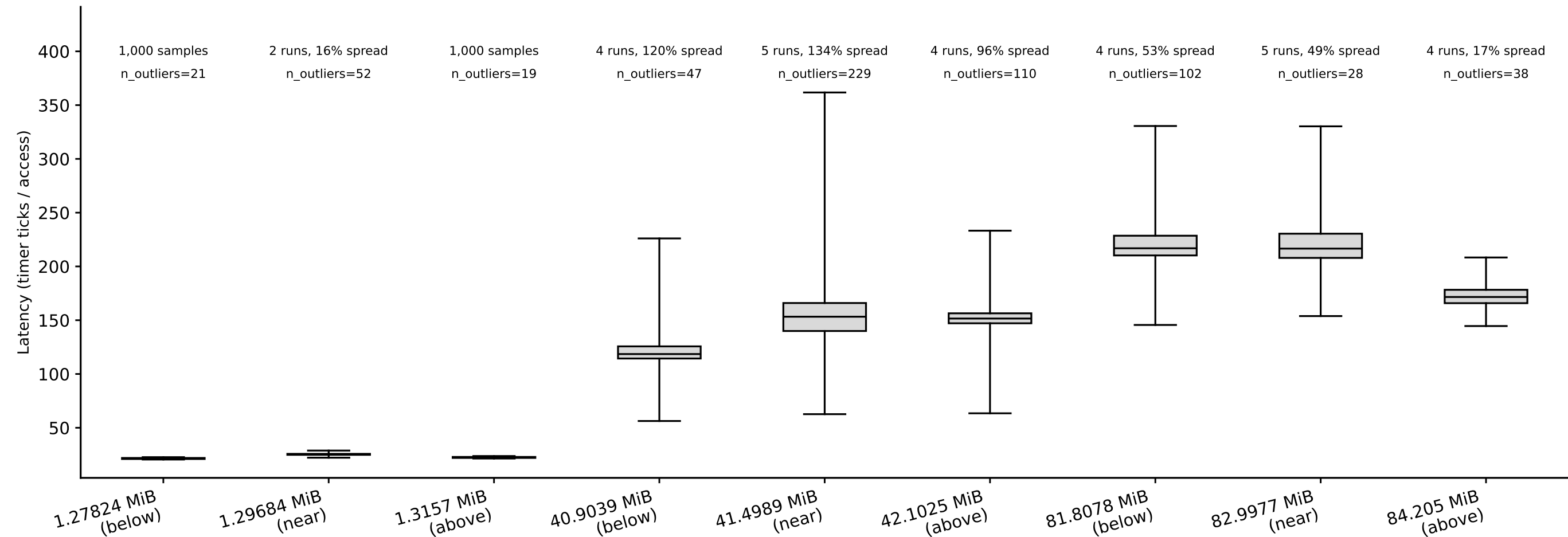
hazel_icelake_8358/capacity_rerun3: capacity box plots, random pattern (whiskers = p5/p95) (Phase I timing-only, auto pipeline) tested boundaries: 1.29684 MiB, 41.4989 MiB, 82.9977 MiB
