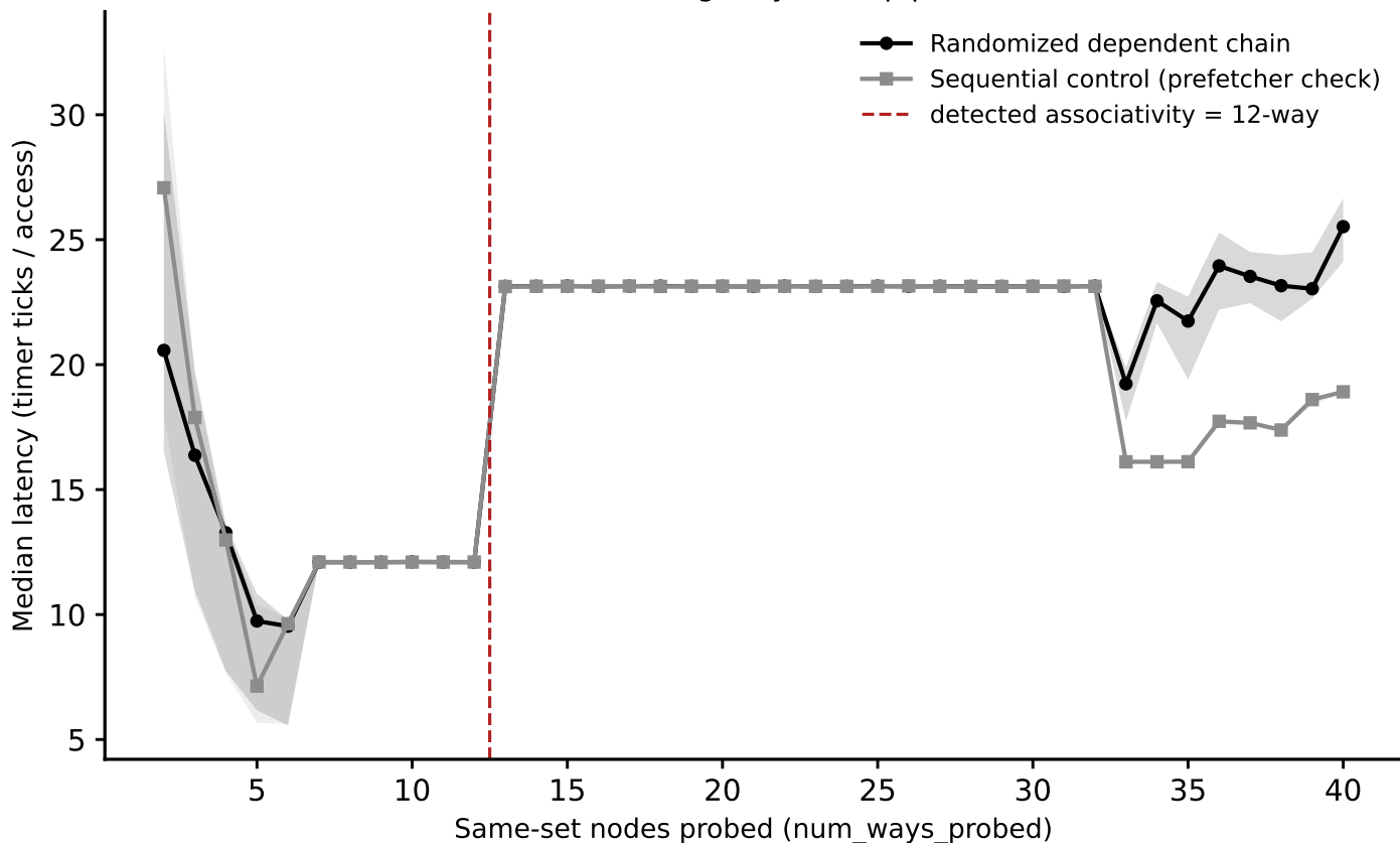
hazel_sapphirerapids/phase1_v2: associativity sweep, L1 (stride=64 KiB) (Phase I timing-only, auto pipeline)
