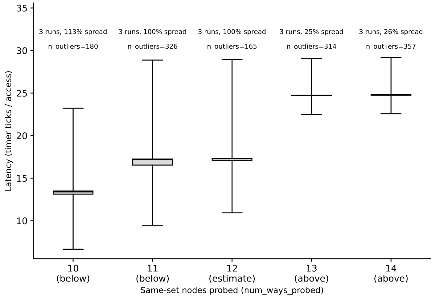
hazel_sapphirerapids/phase1_v2: associativity box plots, L3_LLC, random pattern (whiskers = p5 (Phase I timing-only, auto pipeline) detected associativity estimate: 12-way
