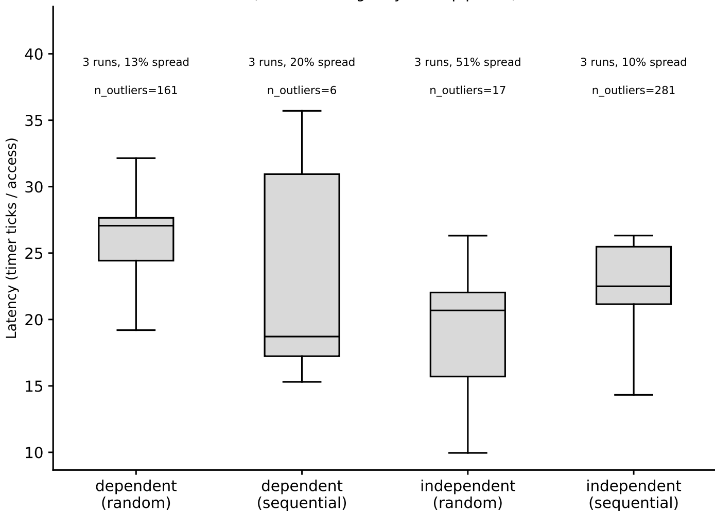
hazel_sapphirerapids/phase1_v2: hit-latency box plots, L1 (footprint=64 KiB) (Phase I timing-only, auto pipeline)
