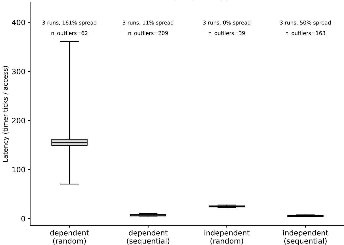
hazel_sapphirerapids/phase1_v2: hit-latency box plots, LLC (footprint=48 MiB) (Phase I timing-only, auto pipeline)
