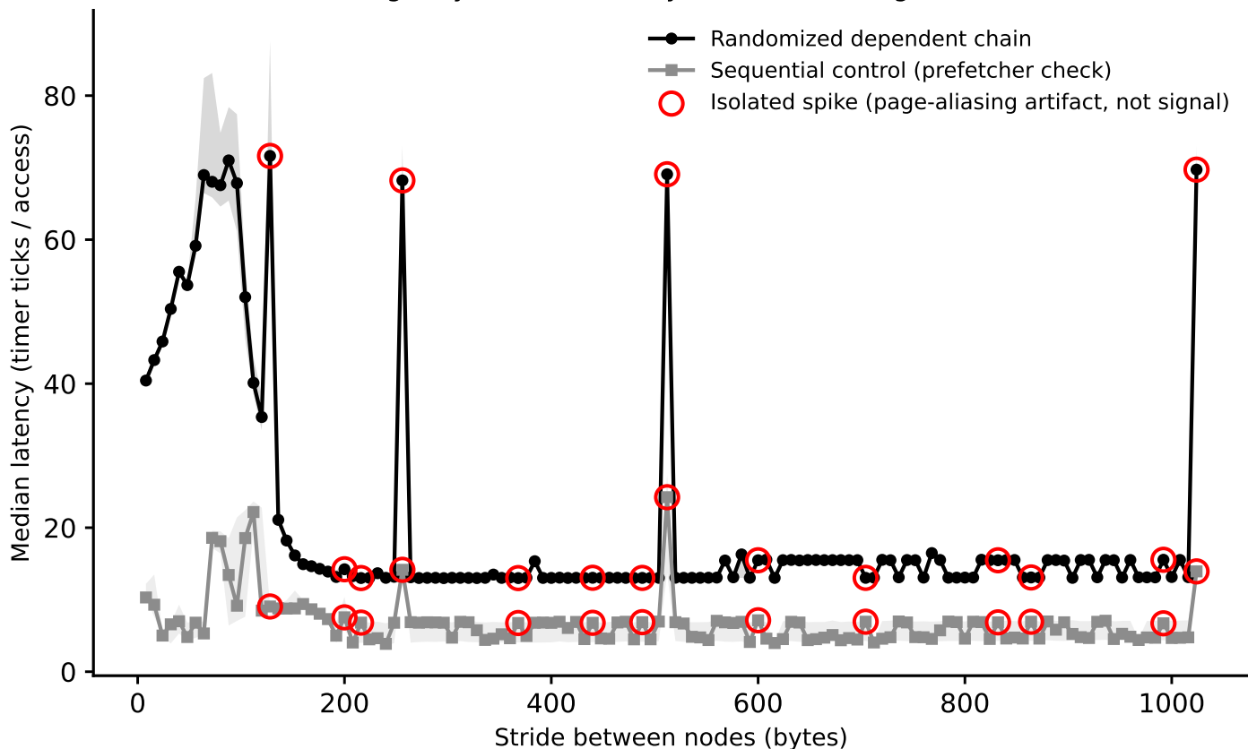
hazel_sapphirerapids/phase1_v2: line-size sweep (dependent pointer chase), footprint=4 MiB (Phase I timing-only, level boundary=2097152B, single-curve method)
