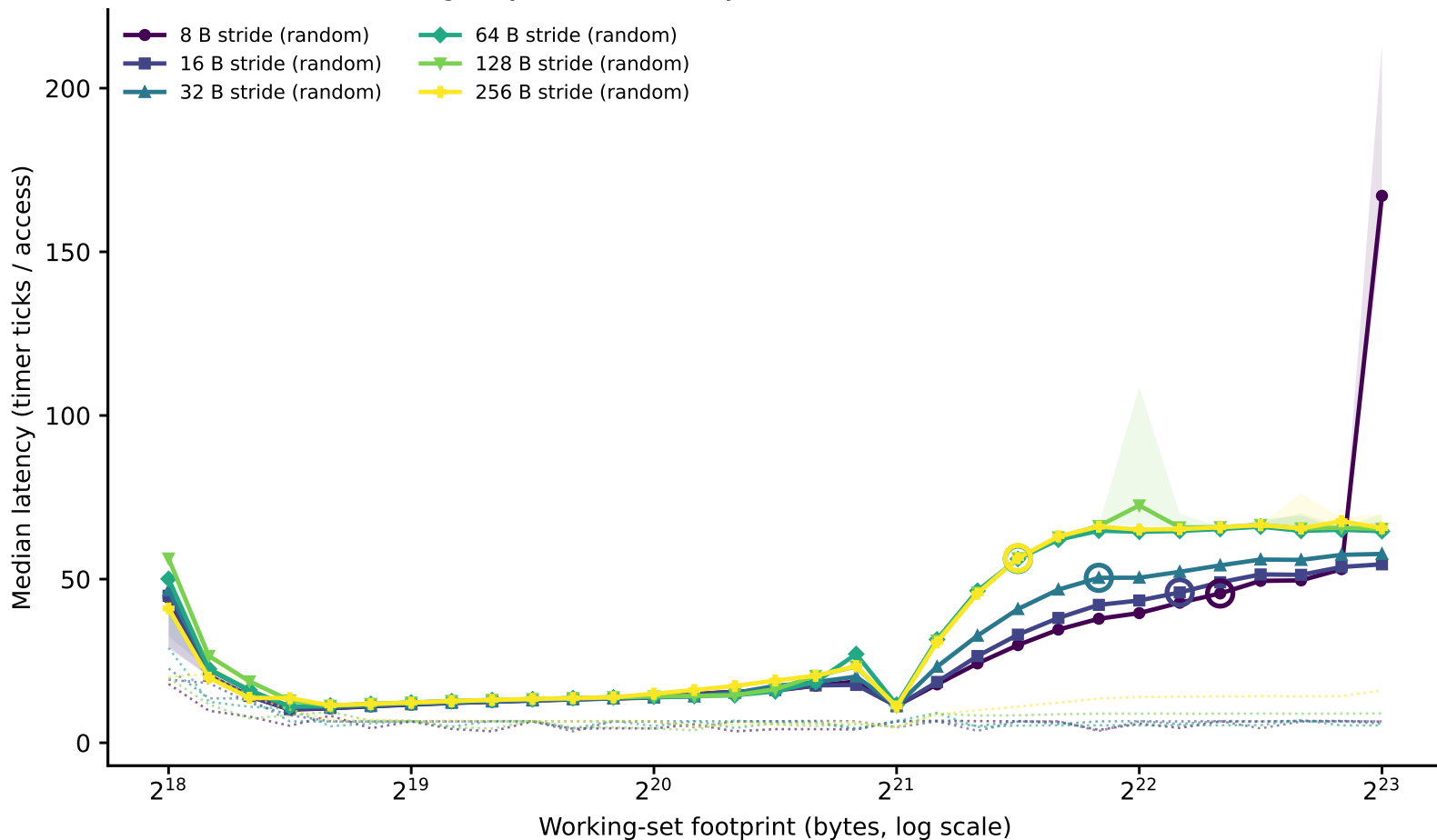
hazel_sapphirerapids/phase1_v2: line-size family of curves (dependent pointer chase) (Phase I timing-only, level boundary=2097152B window=[262144,8388608])
