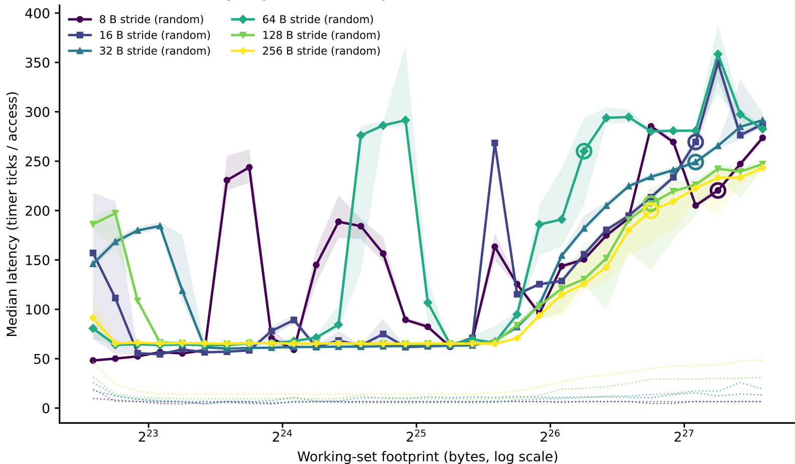
hazel_sapphirerapids/phase1_v2: line-size family of curves (dependent pointer chase) (Phase I timing-only, level boundary=50331648B window=[6291456,201326592])
