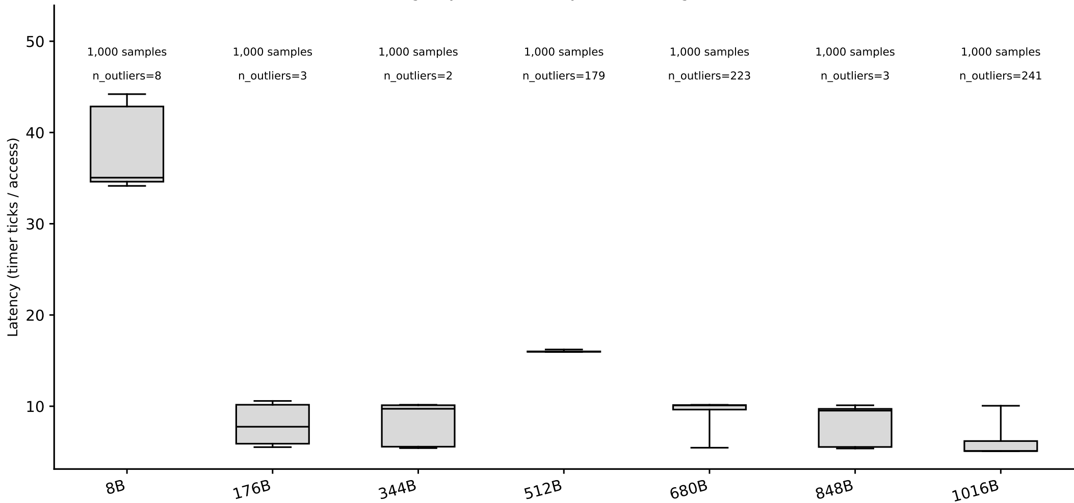
hazel_sapphirerapids/phase1_v2: line-size box plots, random pattern (whiskers = p5/p95) (Phase I timing-only, level boundary=65536B, single-curve method)
