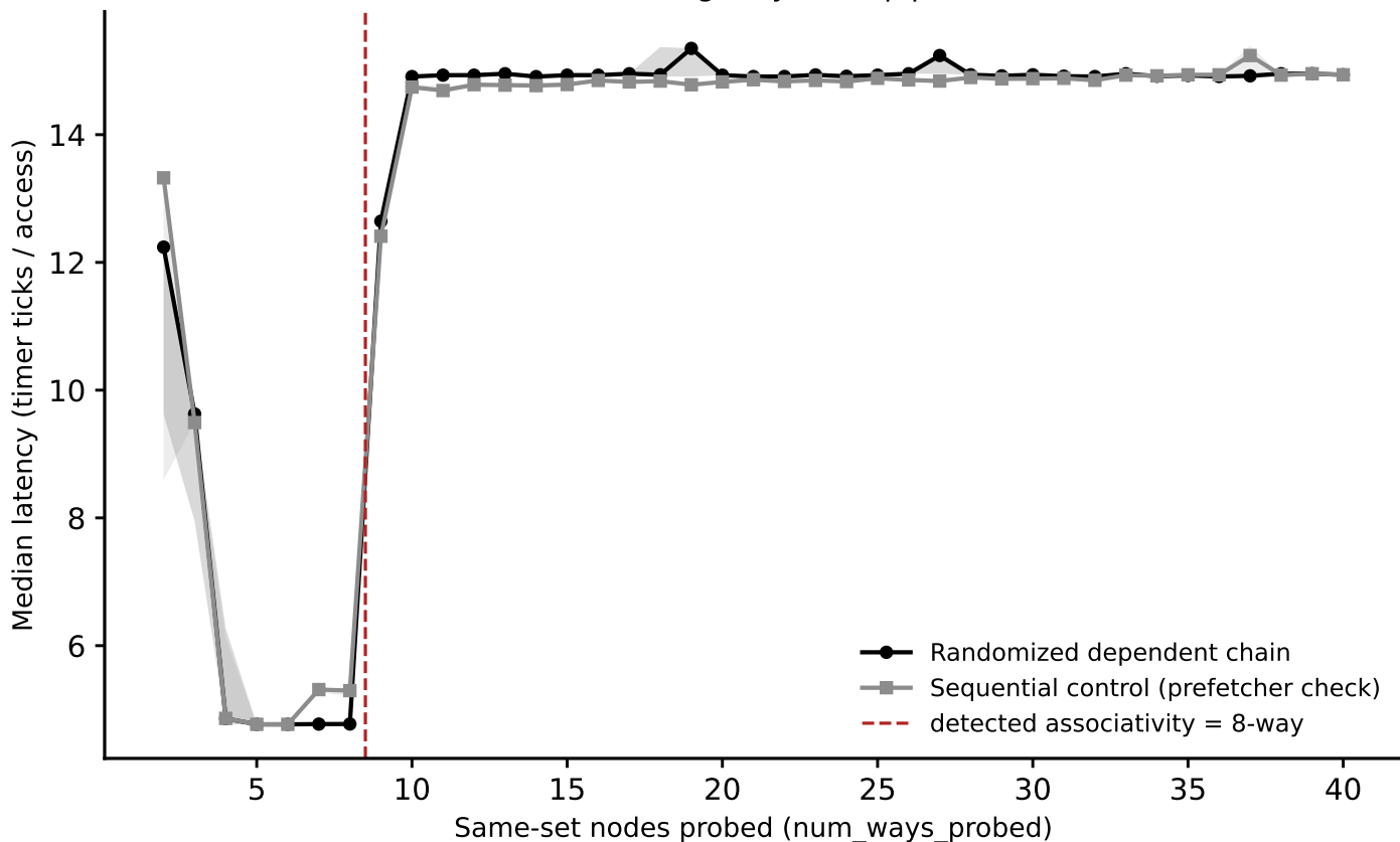
hazel_skylake/phase1_v2: associativity sweep, L1 (stride=32 KiB) (Phase I timing-only, auto pipeline)
