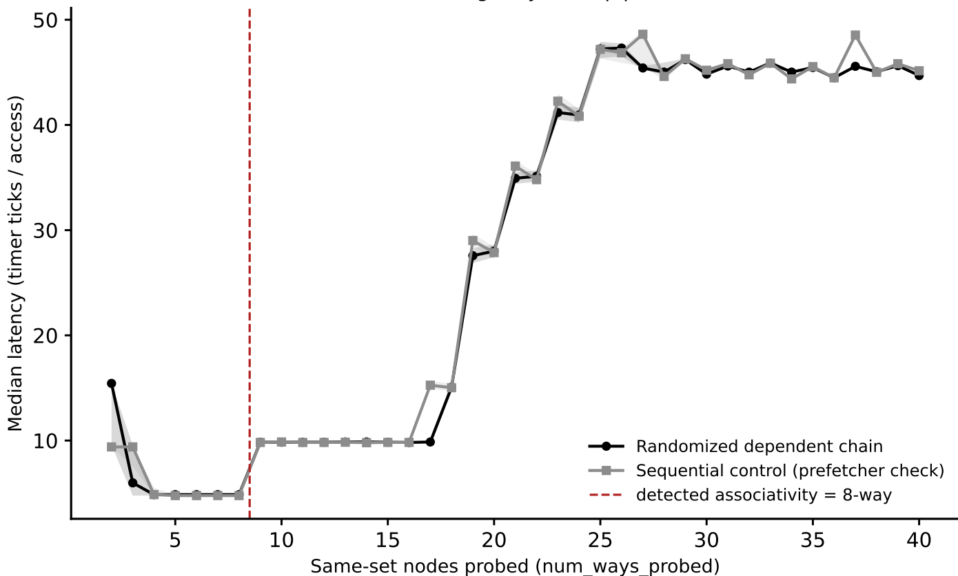
hazel_skylake/phase1_v2: associativity sweep, L2 (stride=1 MiB) (Phase I timing-only, auto pipeline)
