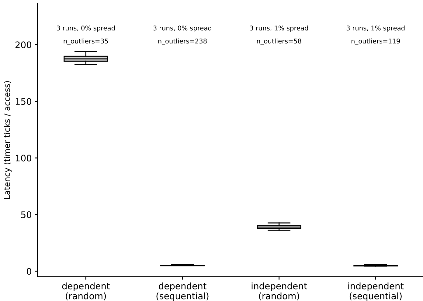
hazel_skylake/phase1_v2: hit-latency box plots, DRAM (footprint=512 MiB) (Phase I timing-only, auto pipeline)
