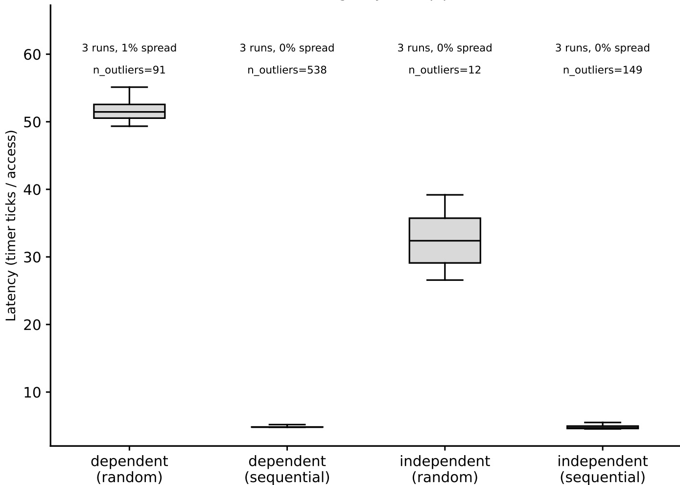
hazel_skylake/phase1_v2: hit-latency box plots, LLC (footprint=22.6274 MiB) (Phase I timing-only, auto pipeline)
