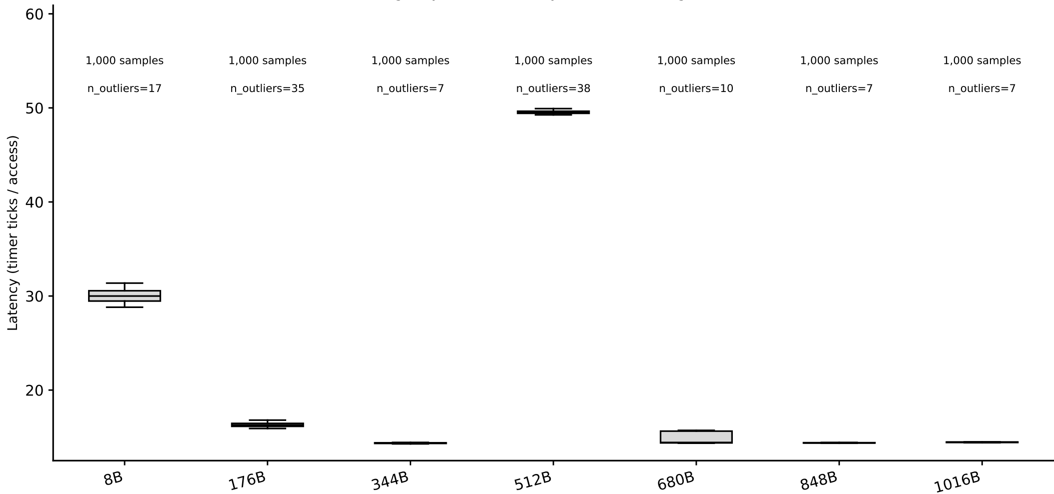
hazel_skylake/phase1_v2: line-size box plots, random pattern (whiskers = p5/p95) (Phase I timing-only, level boundary=1048576B, single-curve method)
