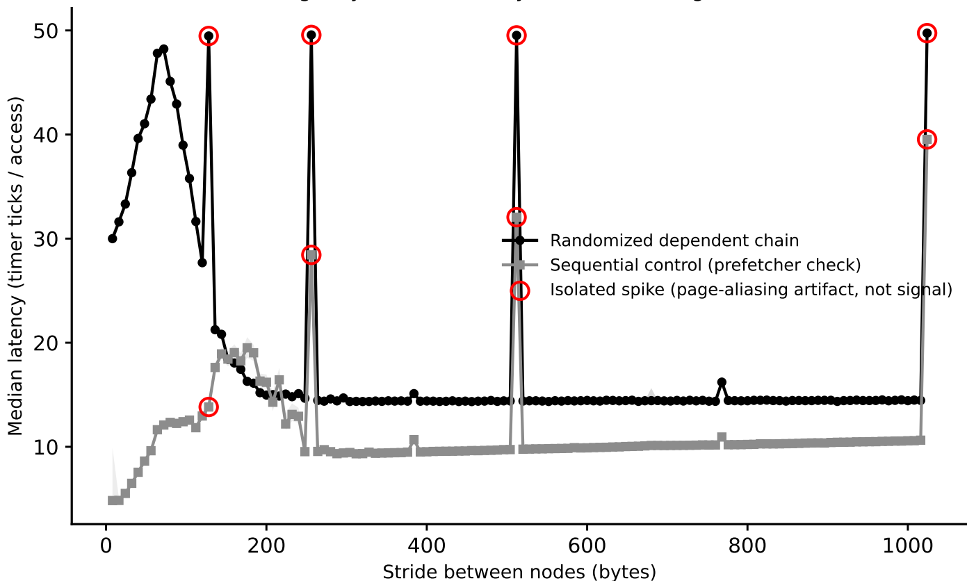
hazel_skylake/phase1_v2: line-size sweep (dependent pointer chase), footprint=2 MiB (Phase I timing-only, level boundary=1048576B, single-curve method)
