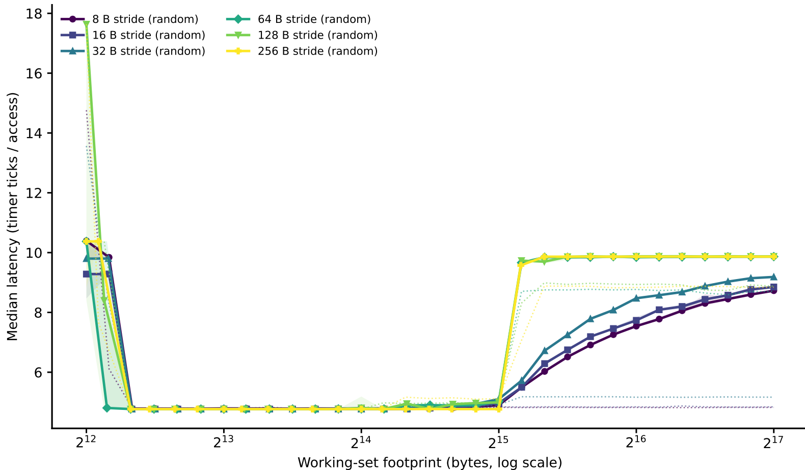
hazel_skylake/phase1_v2: line-size family of curves (dependent pointer chase) (Phase I timing-only, level boundary=32768B window=[4096,131072])
