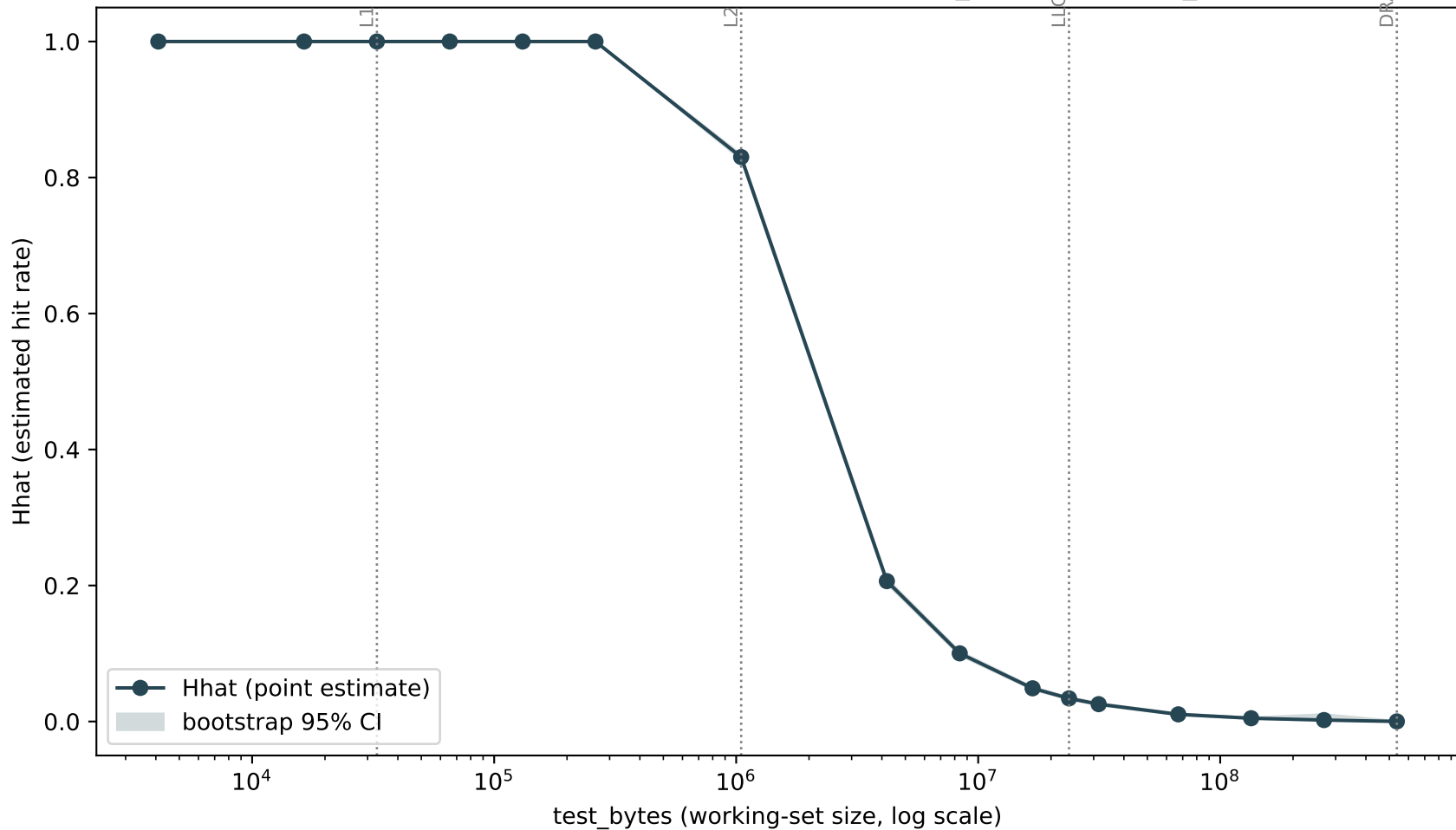
Software-only Hhat vs. working-set size (hazel_skylake/phase1_v2)
