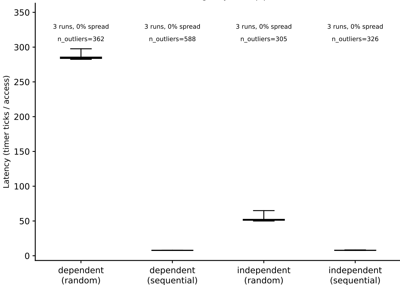
ookay: hit-latency box plots, DRAM (footprint=512 MiB) (Phase I timing-only, auto pipeline)
