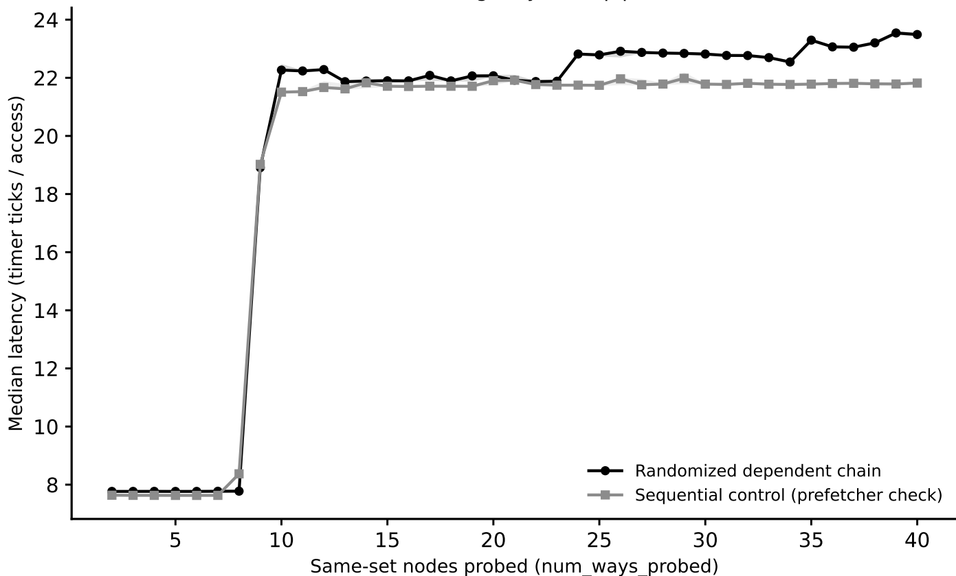
charnwood: associativity sweep, L1 (stride=32 KiB) (Phase I timing-only, auto pipeline)
