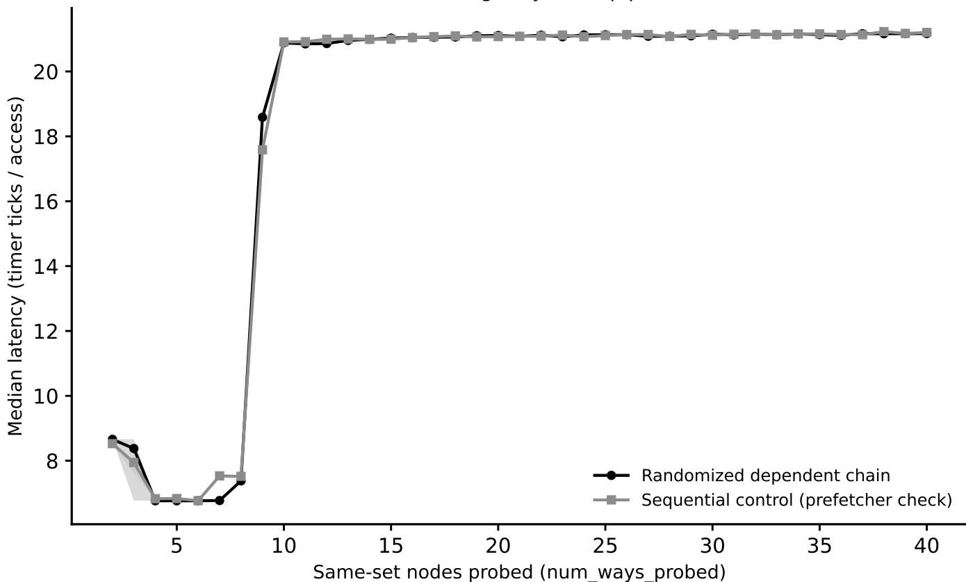
hazel_cascadelake/phase1_v2: associativity sweep, L1 (stride=32 KiB) (Phase I timing-only, auto pipeline)
