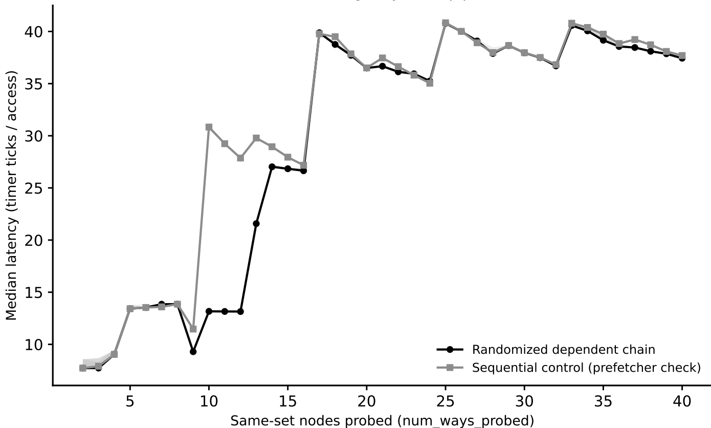
hazel_haswell: associativity sweep, L2 (stride=256 KiB) (Phase I timing-only, auto pipeline)
