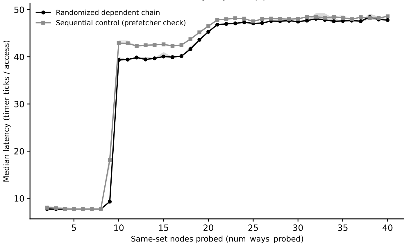
hazel_haswell: associativity sweep, L3_LLC (stride=24 MiB) (Phase I timing-only, auto pipeline)
