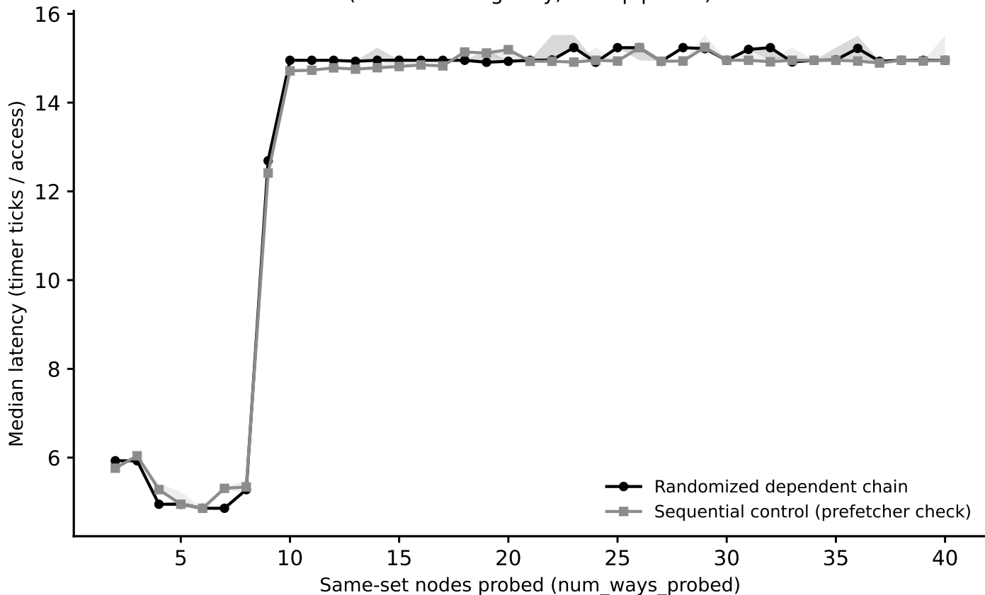
hazel_skylake: associativity sweep, L1 (stride=32 KiB) (Phase I timing-only, auto pipeline)
