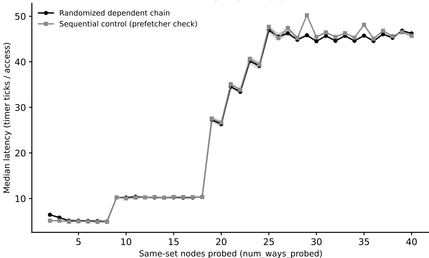
hazel_skylake: associativity sweep, L2 (stride=1 MiB) (Phase I timing-only, auto pipeline)
