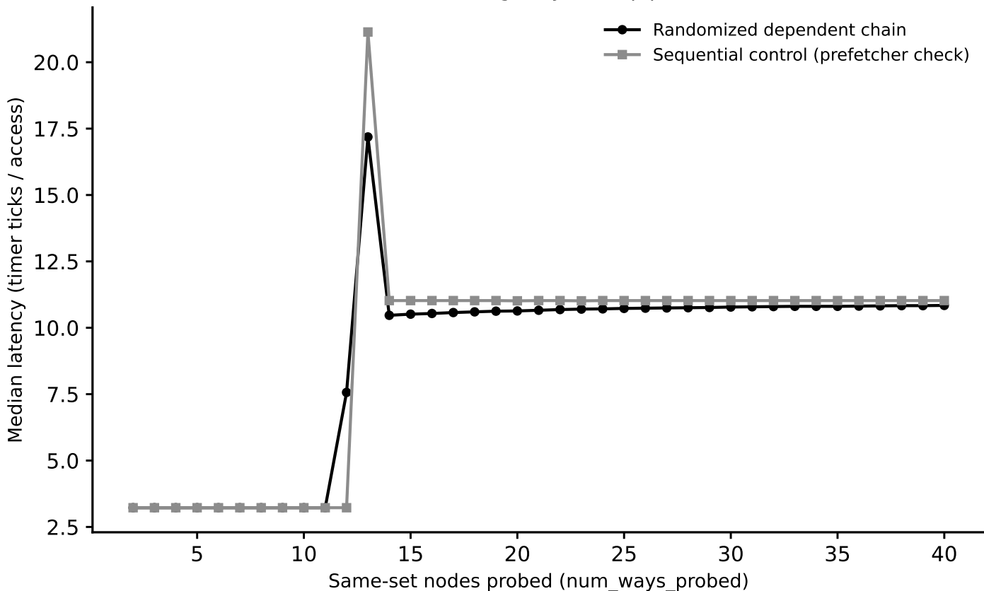
hazel_turin: associativity sweep, L3_LLC (stride=32 MiB) (Phase I timing-only, auto pipeline)
