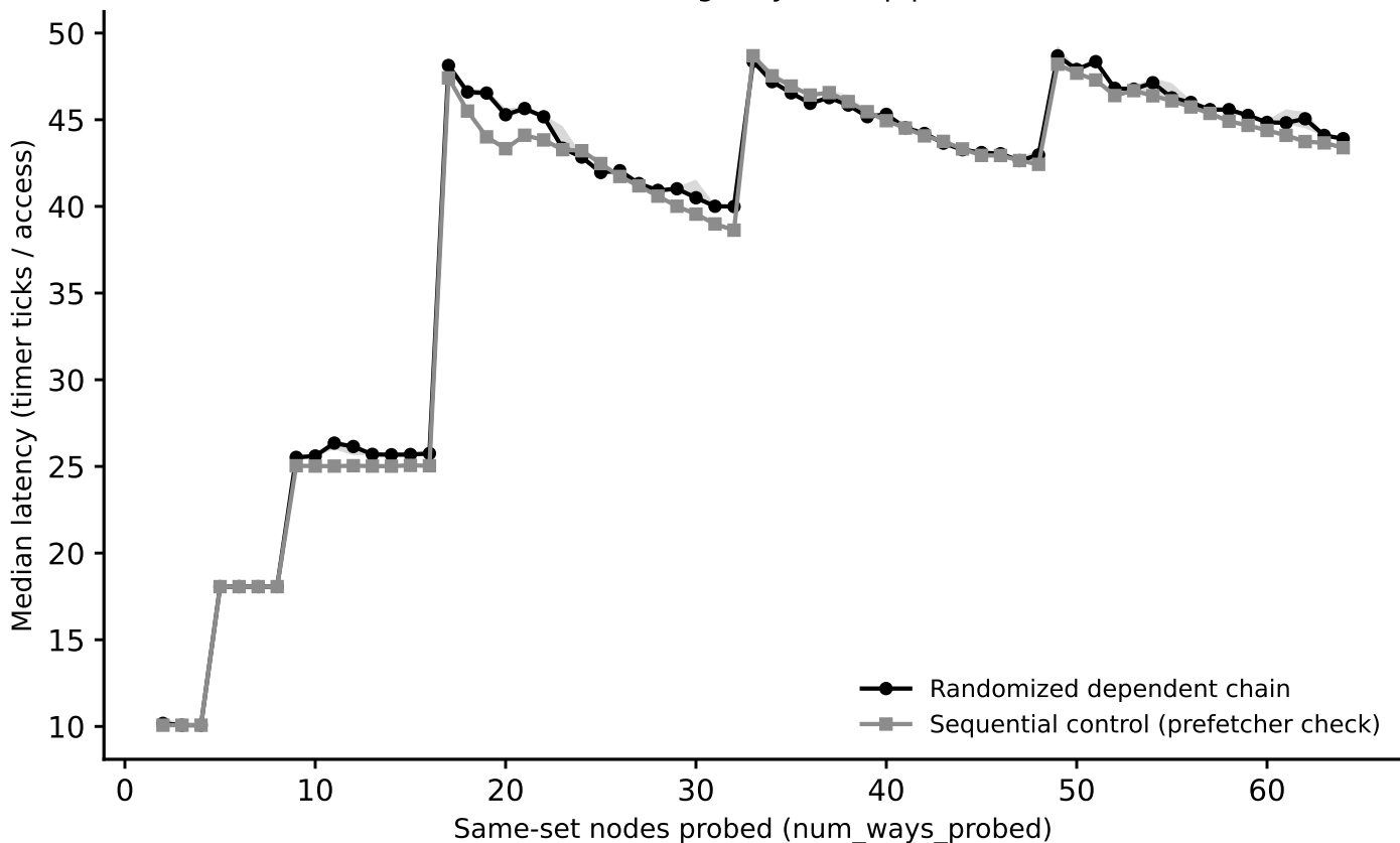
sunbird: associativity sweep, L2_128KiB_candidate (stride=128 KiB) (Phase I timing-only, auto pipeline)
