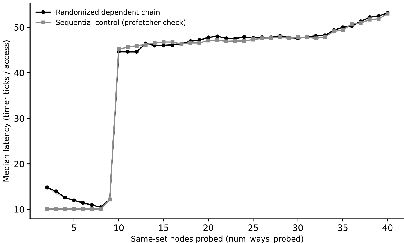
sunbird: associativity sweep, L3_LLC (stride=30 MiB) (Phase I timing-only, auto pipeline)
