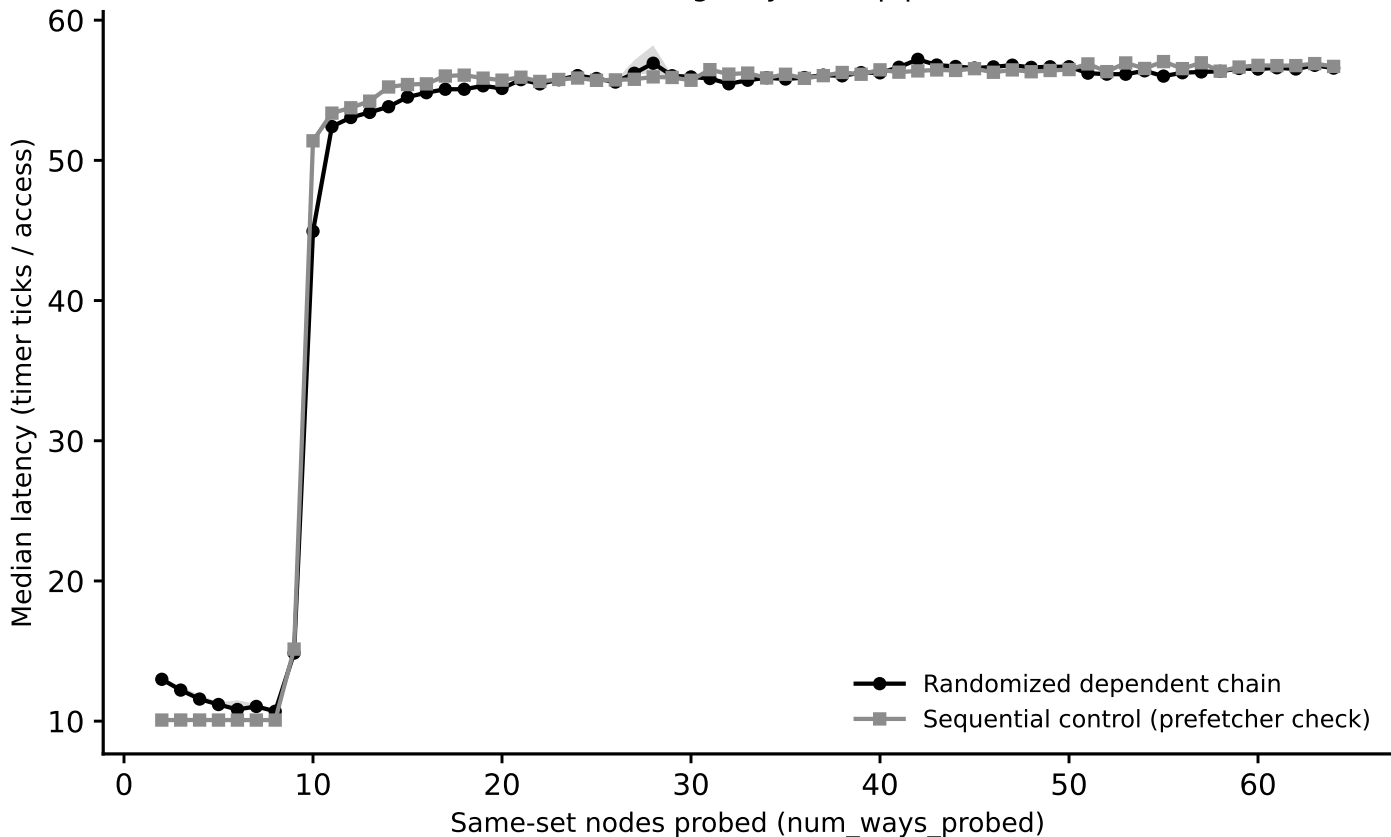
sunbird: associativity sweep, LLC_16MiB (stride=16 MiB) (Phase I timing-only, auto pipeline)
