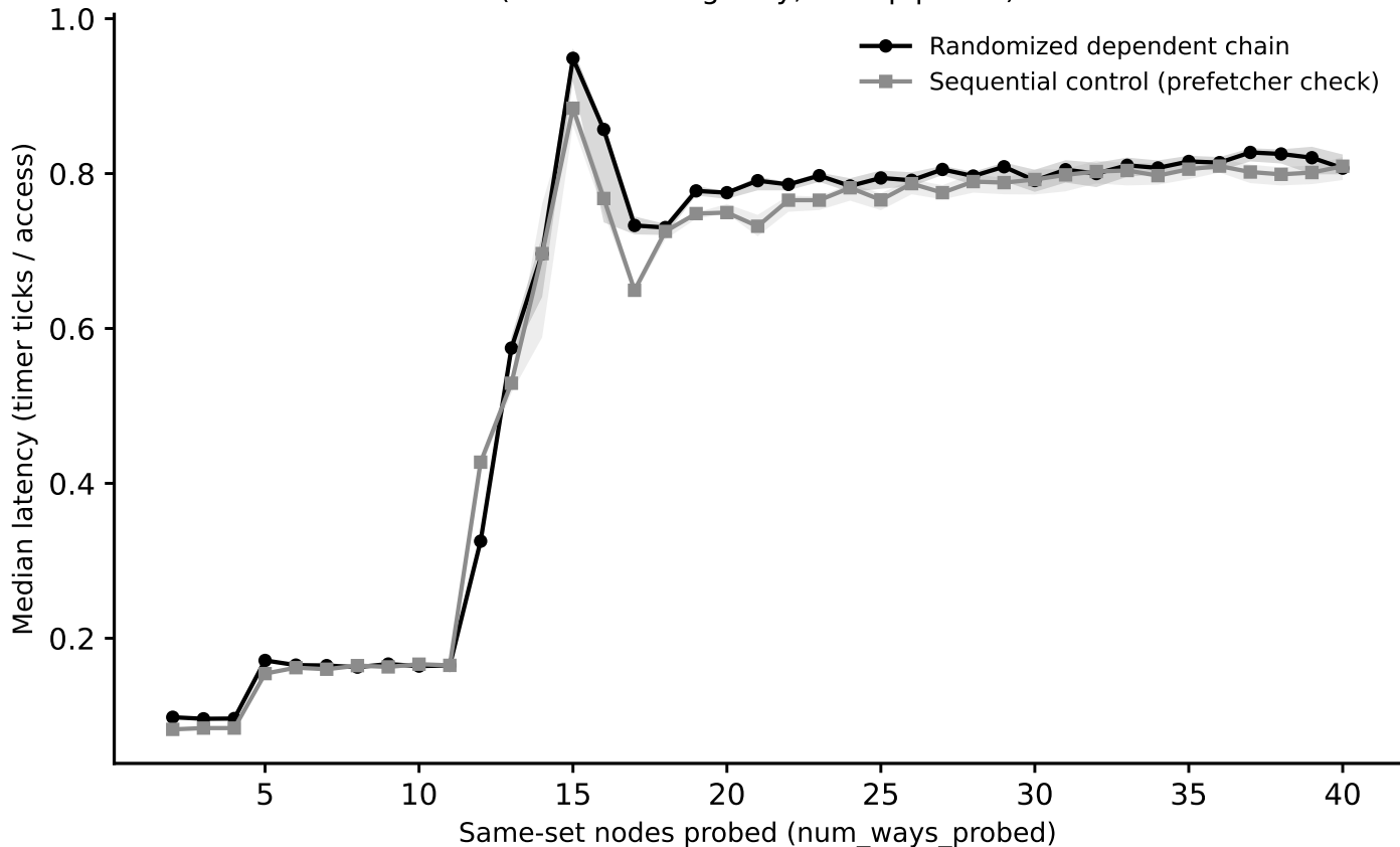
thunderbird: associativity sweep, L2 (stride=1 MiB) (Phase I timing-only, auto pipeline)
