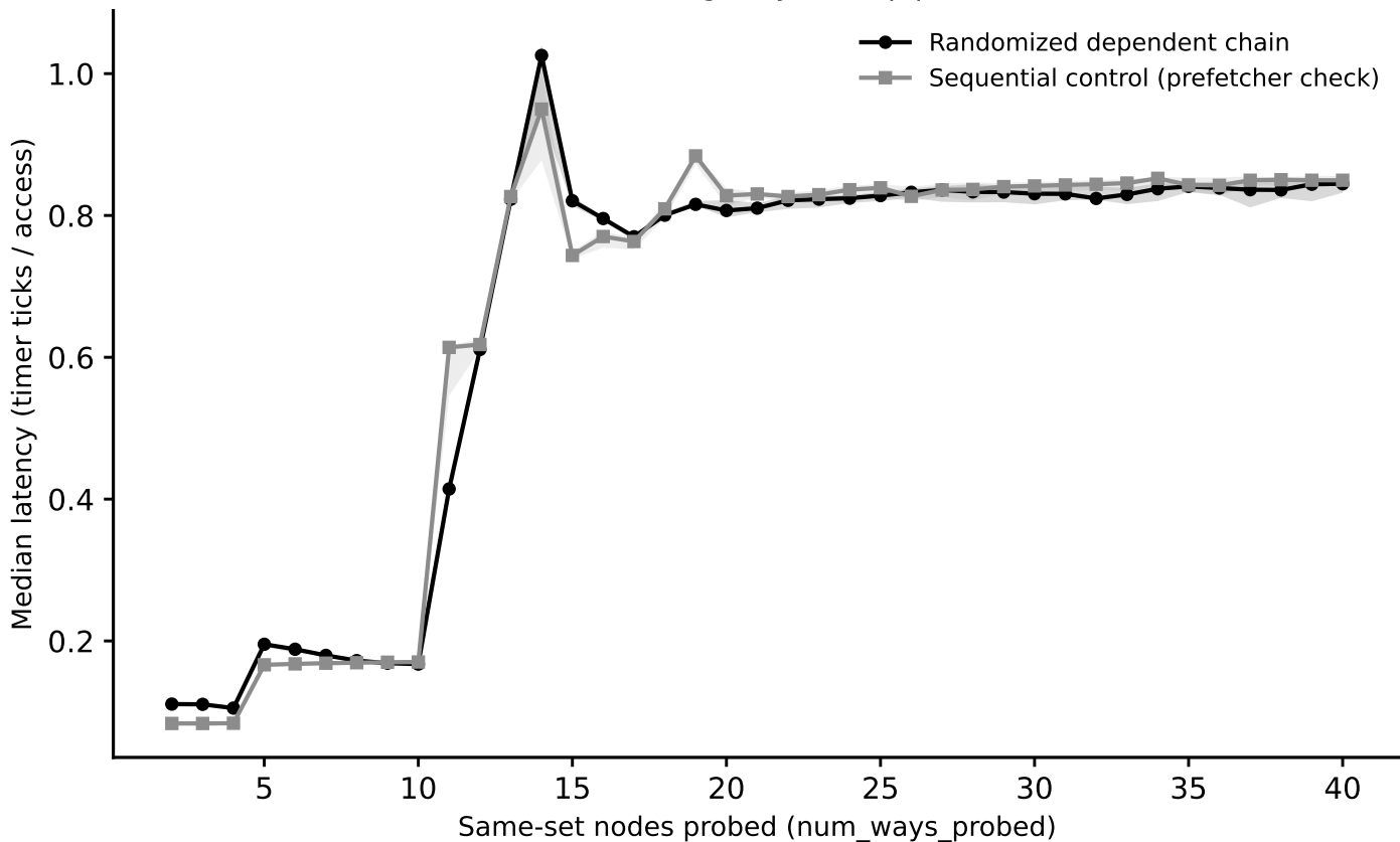
thunderbird: associativity sweep, L3_LLC (stride=30 MiB) (Phase I timing-only, auto pipeline)
