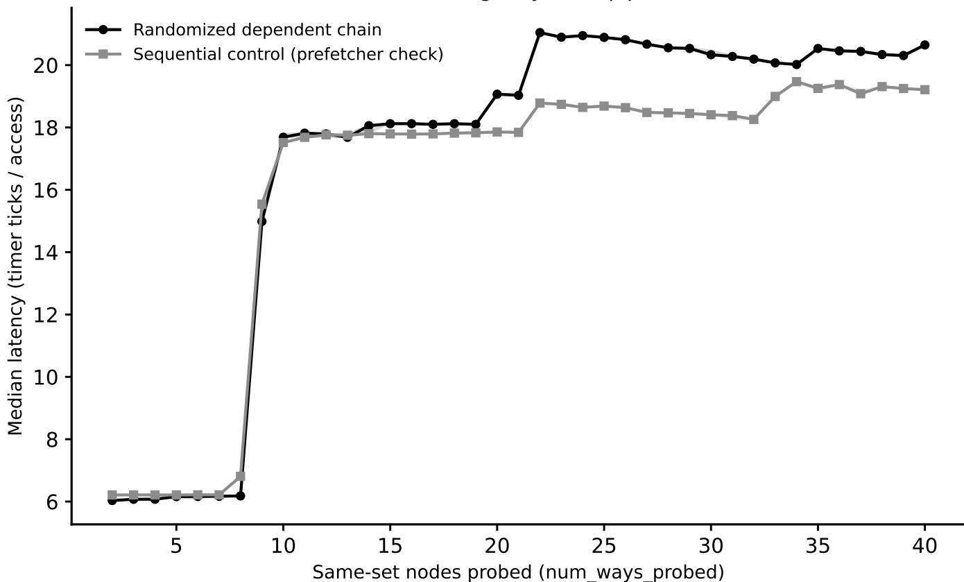
upgrade: associativity sweep, L1 (stride=32 KiB) (Phase I timing-only, auto pipeline)
