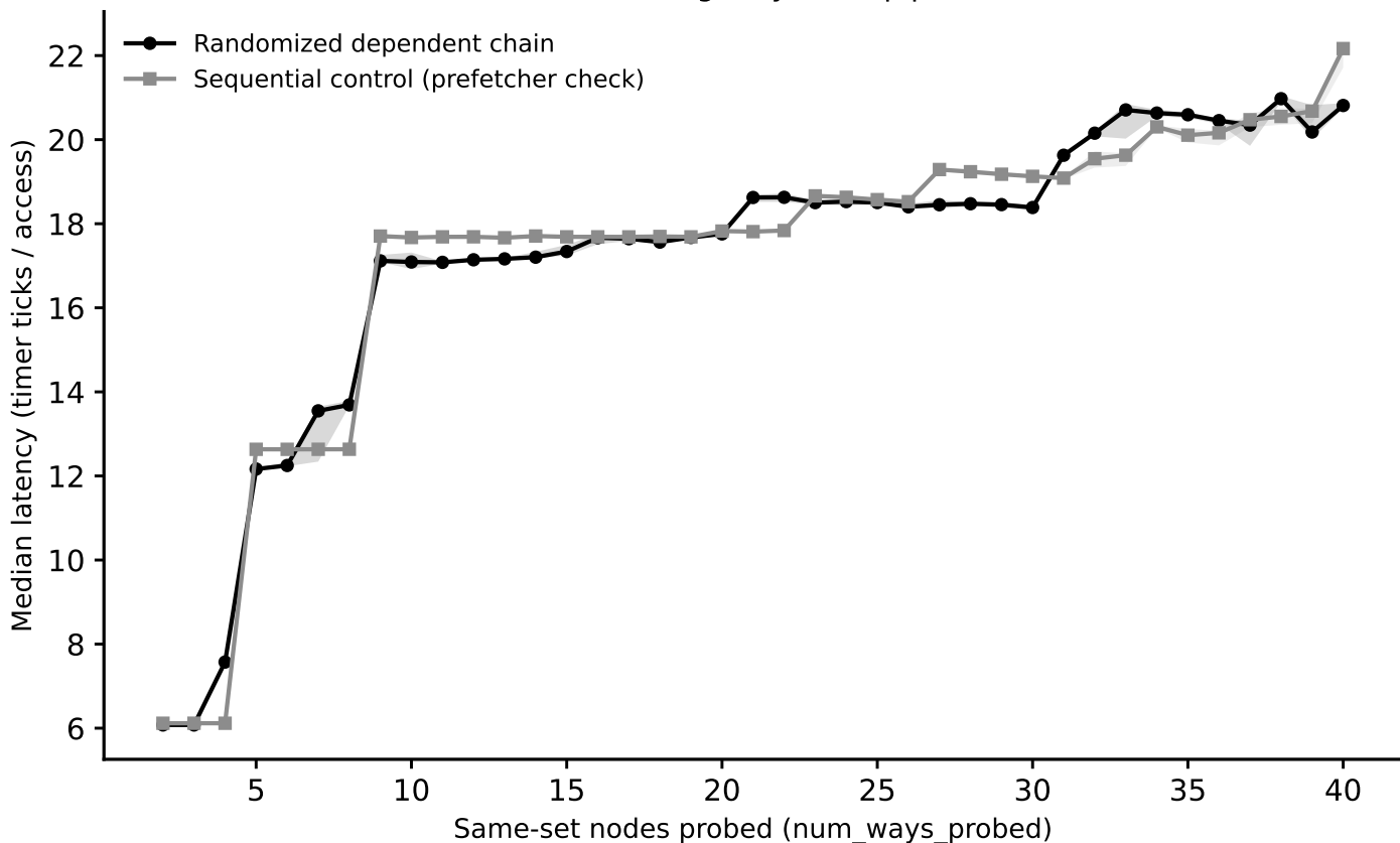
upgrade: associativity sweep, L3_LLC (stride=16 MiB) (Phase I timing-only, auto pipeline)
