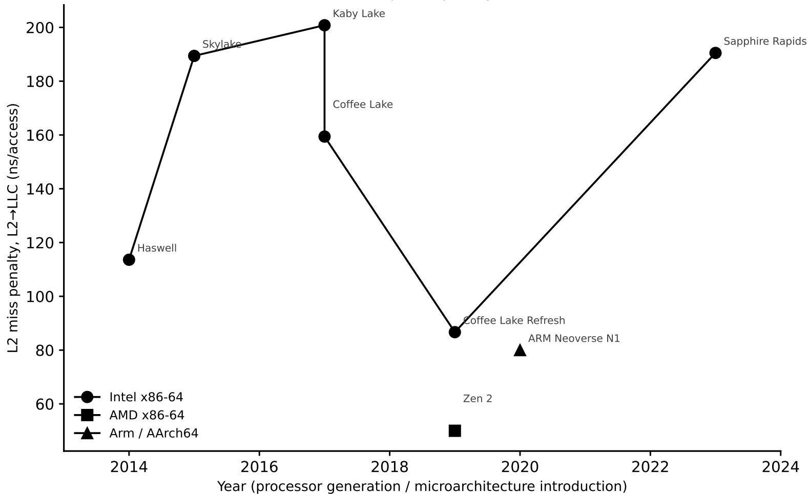
L2 miss penalty vs. year
