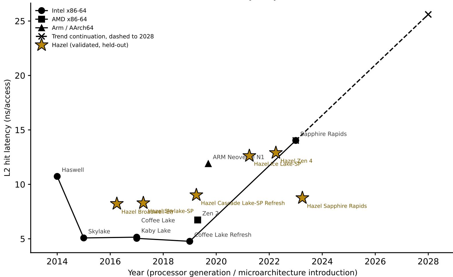
L2 hit latency vs. year
