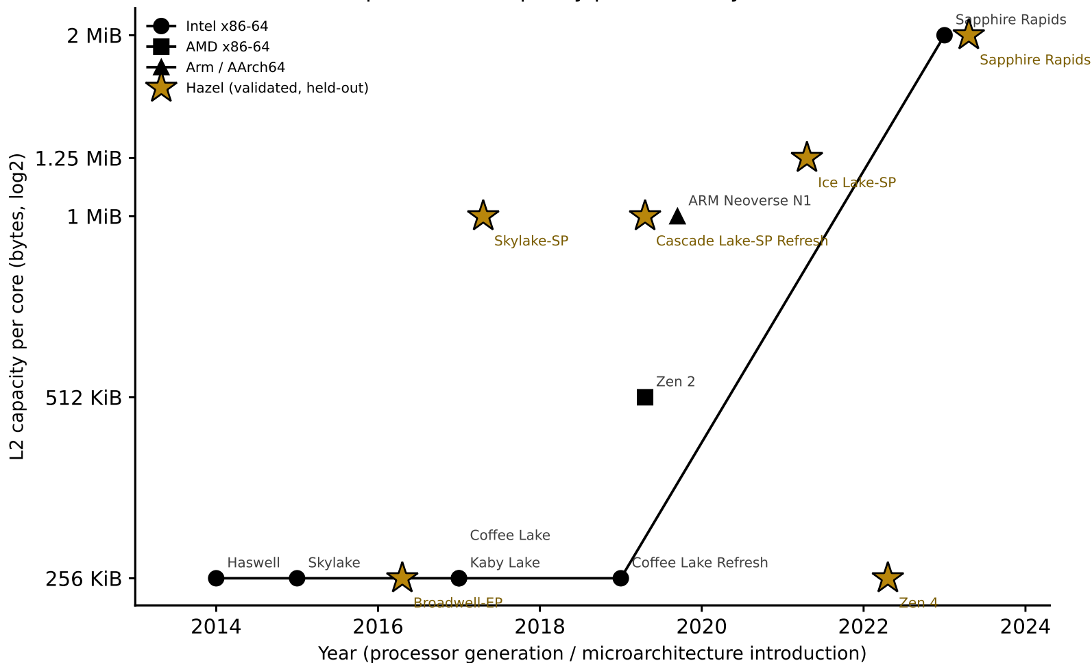
Final combined comparison: L2 capacity per core vs. year (lab + validated Hazel)
