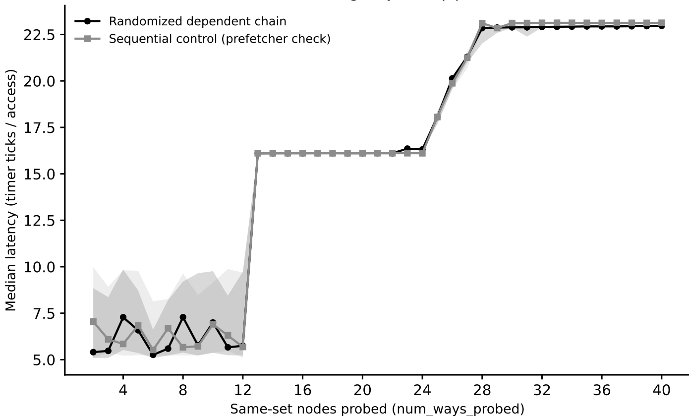
artemisia: associativity sweep, L1 (stride=48 KiB) (Phase I timing-only, auto pipeline)
