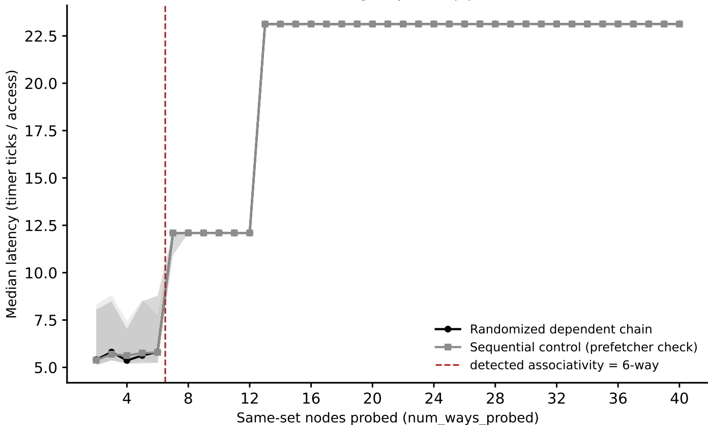
artemisia: associativity sweep, L3_LLC (stride=30 MiB) (Phase I timing-only, auto pipeline)
