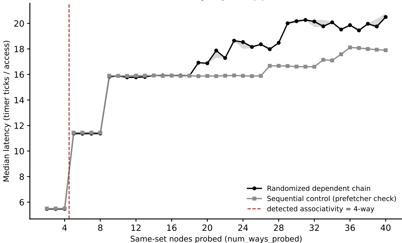
crux: associativity sweep, L2 (stride=256 KiB) (Phase I timing-only, auto pipeline)
