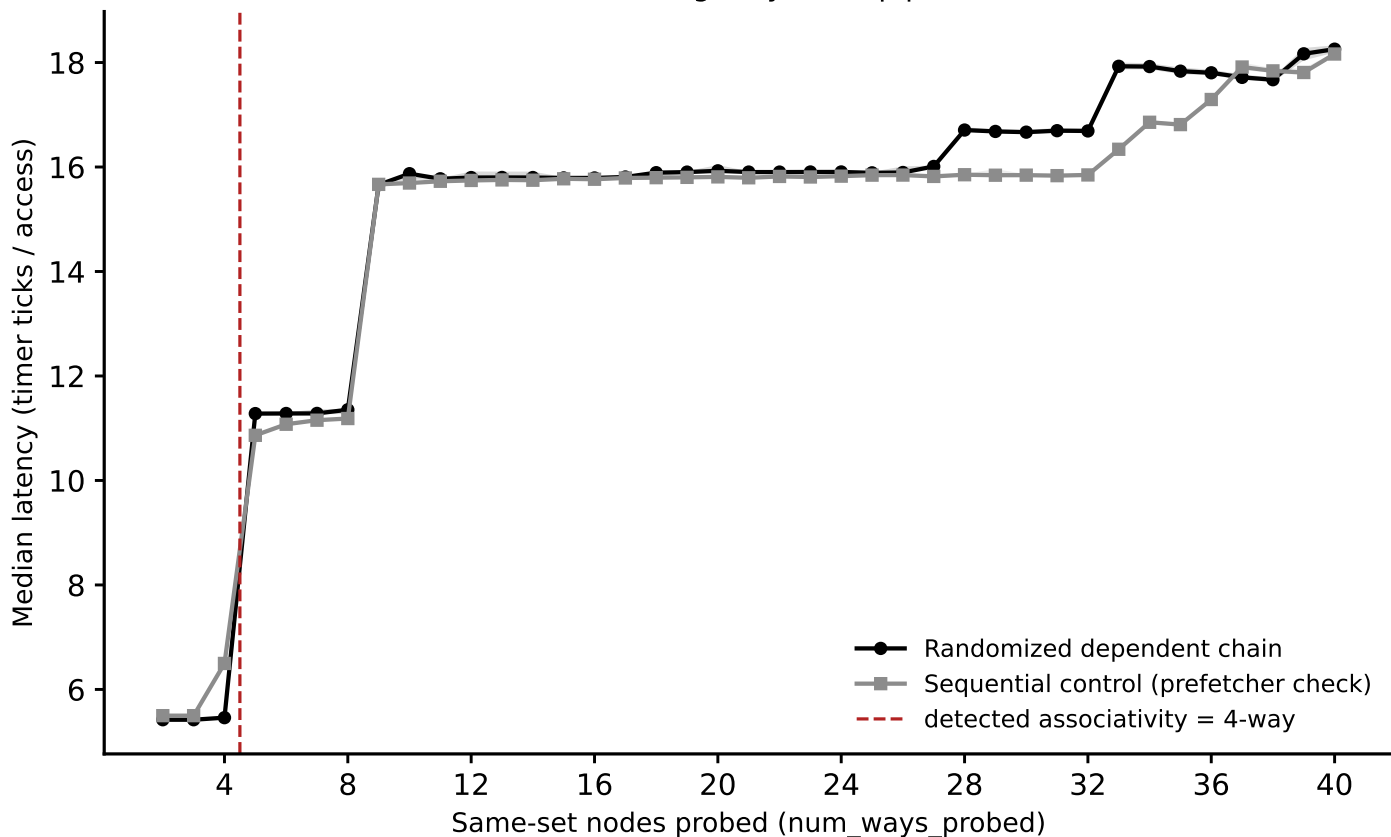
crux: associativity sweep, L3_LLC (stride=8 MiB) (Phase I timing-only, auto pipeline)
