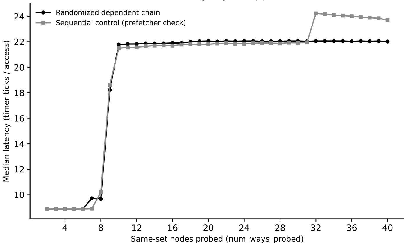
hazel_broadwell: associativity sweep, L1 (stride=32 KiB) (Phase I timing-only, auto pipeline)
