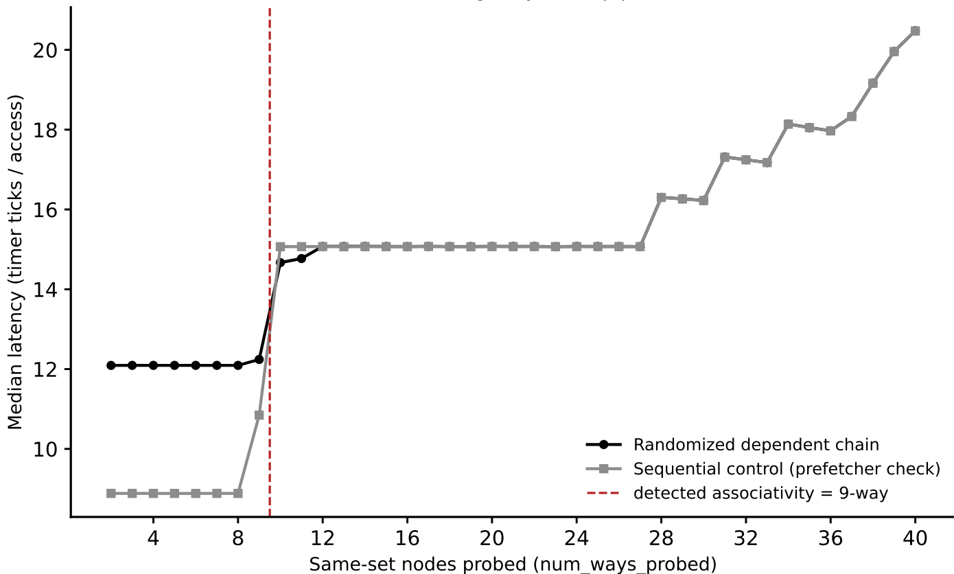
hazel_broadwell: associativity sweep, L3_LLC (stride=24.6758 MiB) (Phase I timing-only, auto pipeline)
