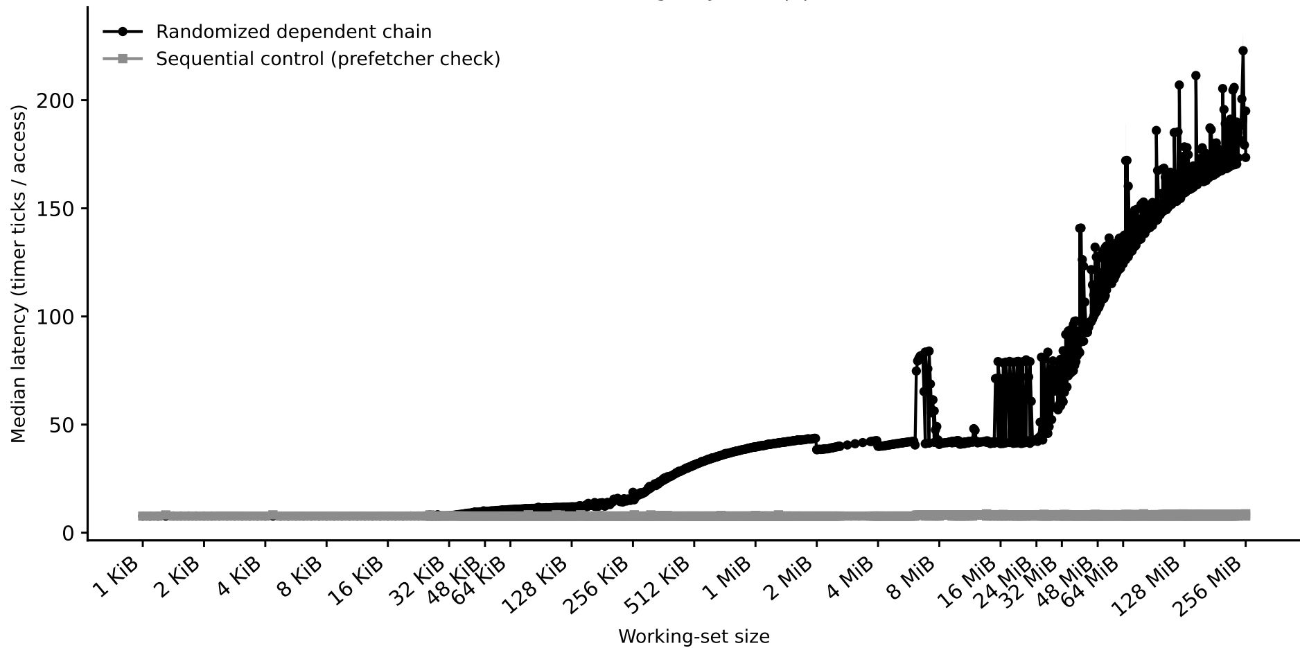
hazel_broadwell: capacity sweep (dependent pointer chase) (Phase I timing-only, auto pipeline)
