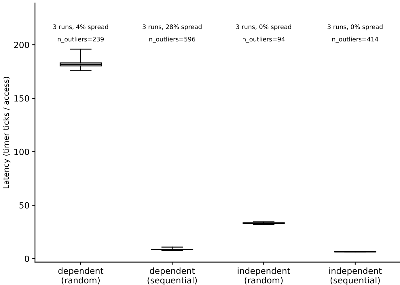
hazel_broadwell: hit-latency box plots, DRAM (footprint=512 MiB) (Phase I timing-only, auto pipeline)
