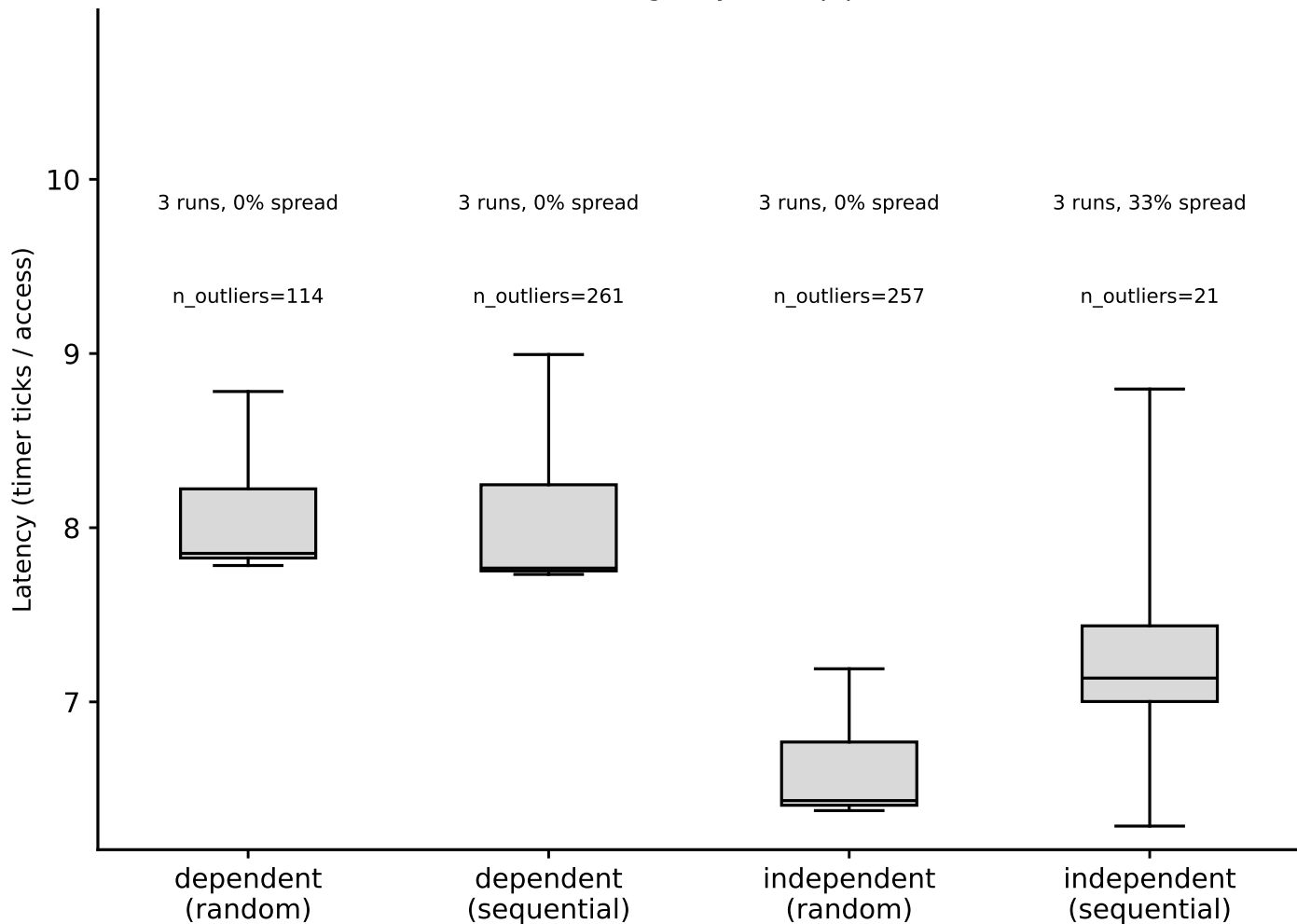
hazel_broadwell: hit-latency box plots, L1 (footprint=32 KiB) (Phase I timing-only, auto pipeline)
