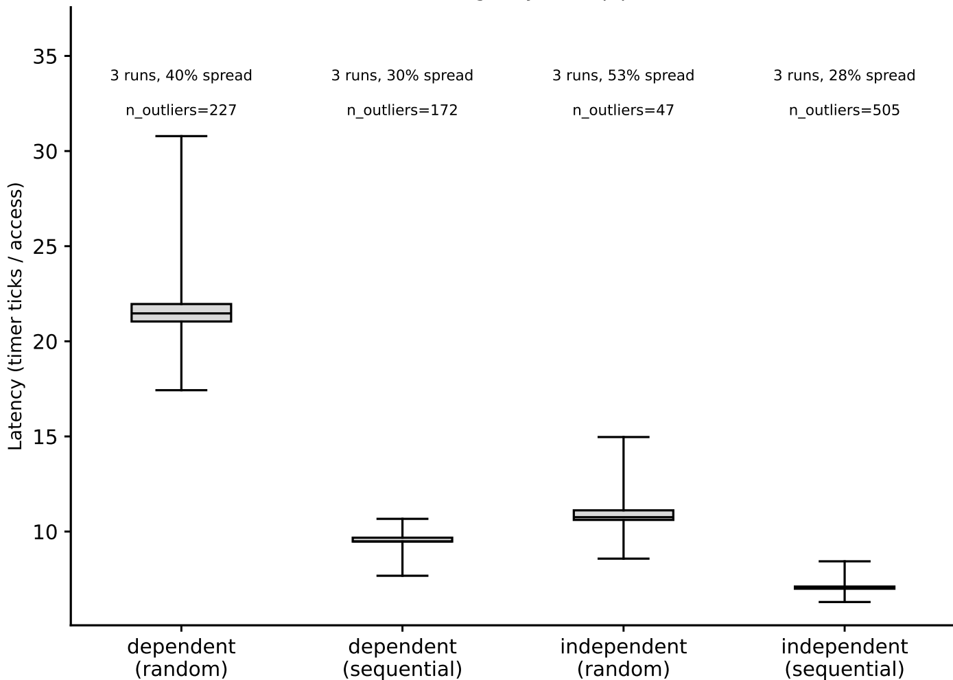
hazel_broadwell: hit-latency box plots, L2 (footprint=256 KiB) (Phase I timing-only, auto pipeline)
